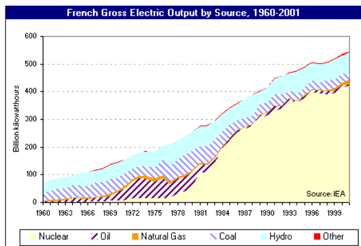
Fig. 1: French electrical output by source (Source: DOE)
